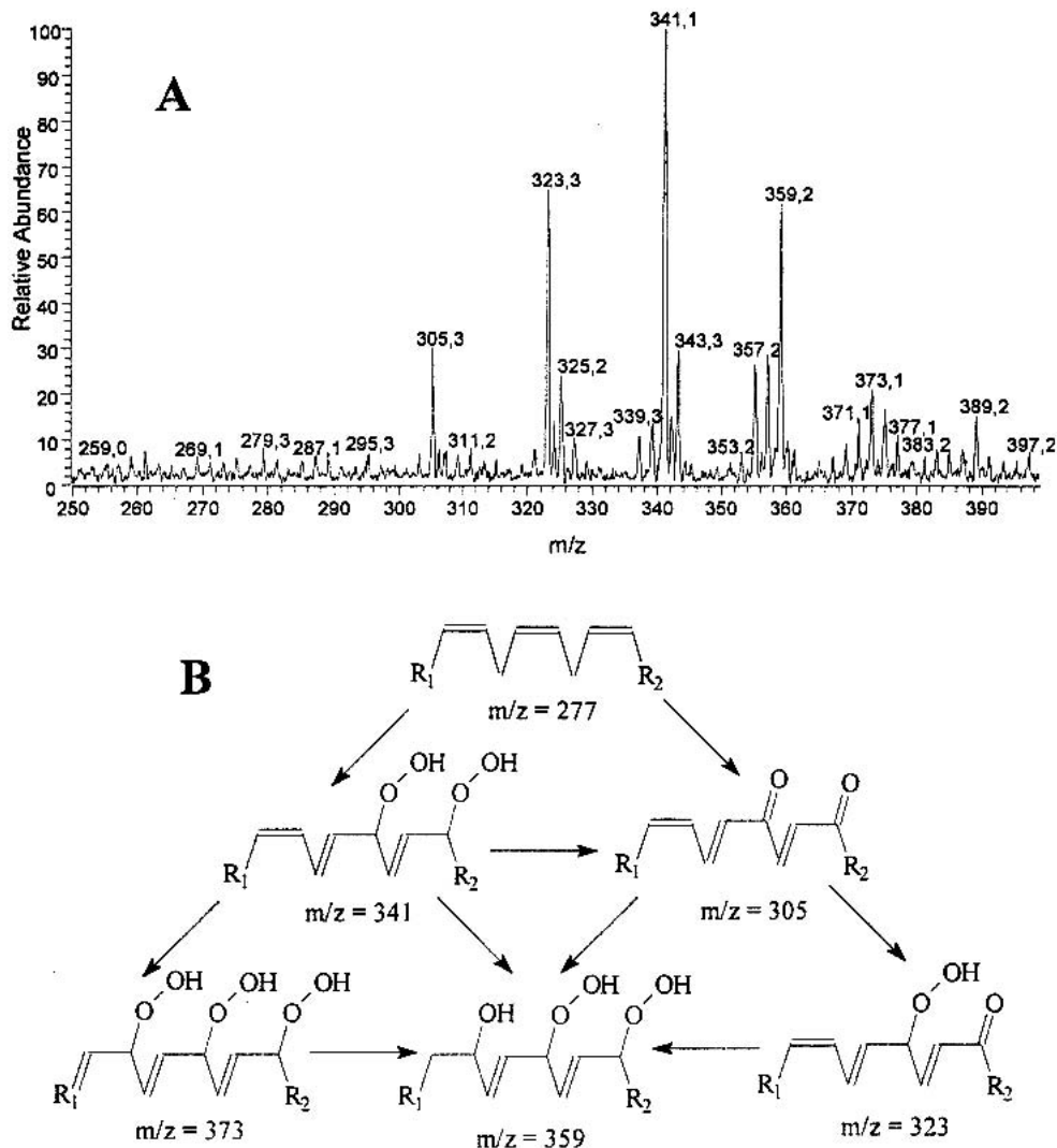
Fig. 3. (A) Negative ion mode ESI mass spectrum of linolenic acid irradiated with 0.25 \text{ J/cm}^2 UV-B in the presence of 10 \mu\text{M Fe(II)} . (B) Scheme of some of the possible lipid peroxidation products of linolenic acid.
